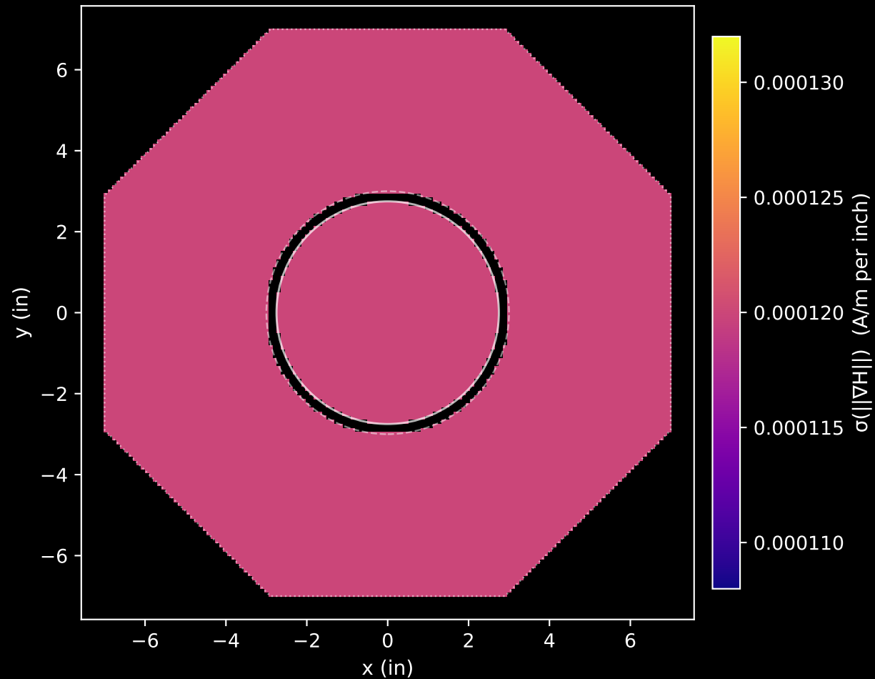
Propagated uncertainty
